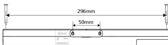
Fixed Mount
