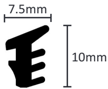
P40 Wedge
