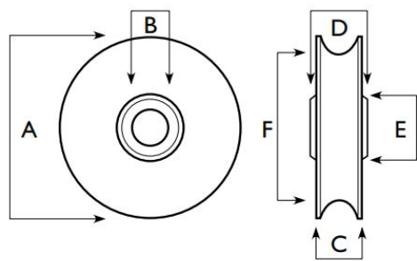
Rollers with Bores
