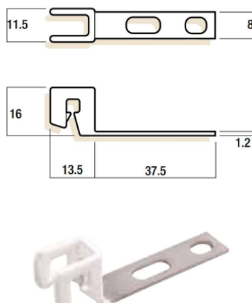
Adjustable Foot
