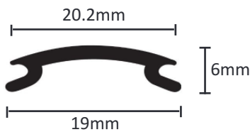
Wardrobe Infill
