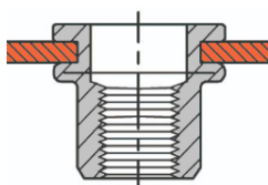
Large Flange Rivnut
