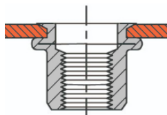
Low Profile Rivnut
