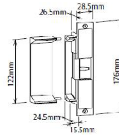
ES9000 with 50mm Extension Lip
