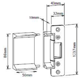
ES110 with 50mm ext lip - "A" Plate
