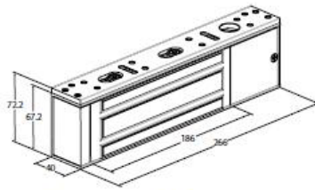
Z8 Electromagnetic Lock
