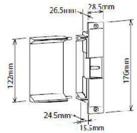
ES9000 with 75mm Extension Lip
