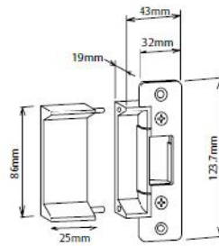
ES110 with 25mm ext lip - "A" Plate
