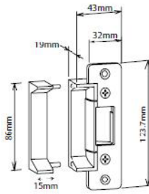
ES110 with 15mm ext lip - "A" Plate
