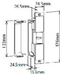
ES9000 with 25mm Extension Lip
